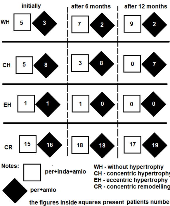
Figure 5: The dynamics of AH patient number with absence and different types of LV remodeling during antihypertensive therapy
